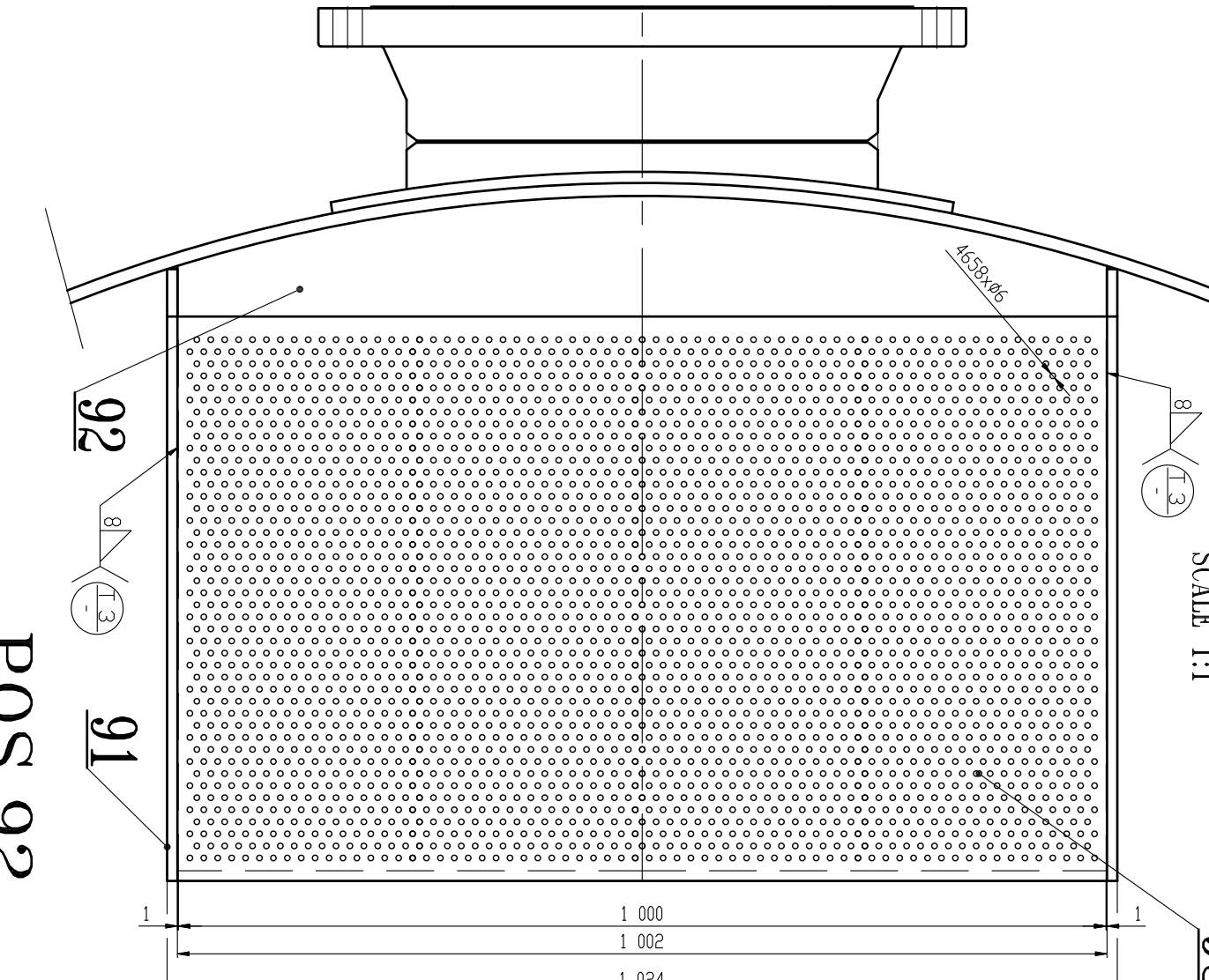
VIEW R WIDOK R
